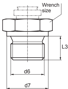
Cylindrical screw threads
